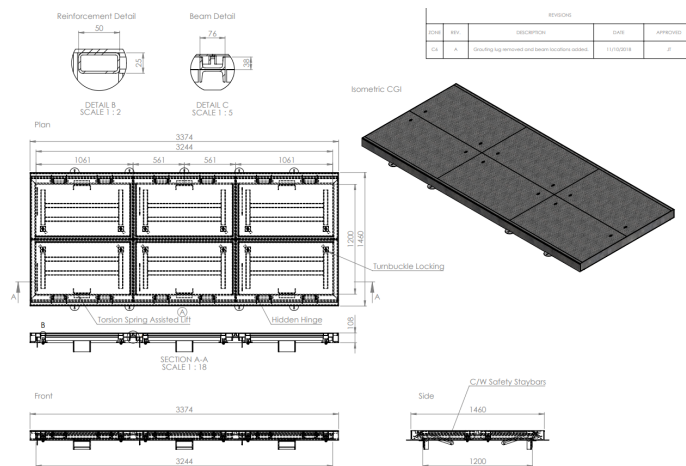
Typical approval drawing
