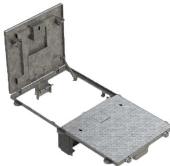
Twin lid with padlock facility
